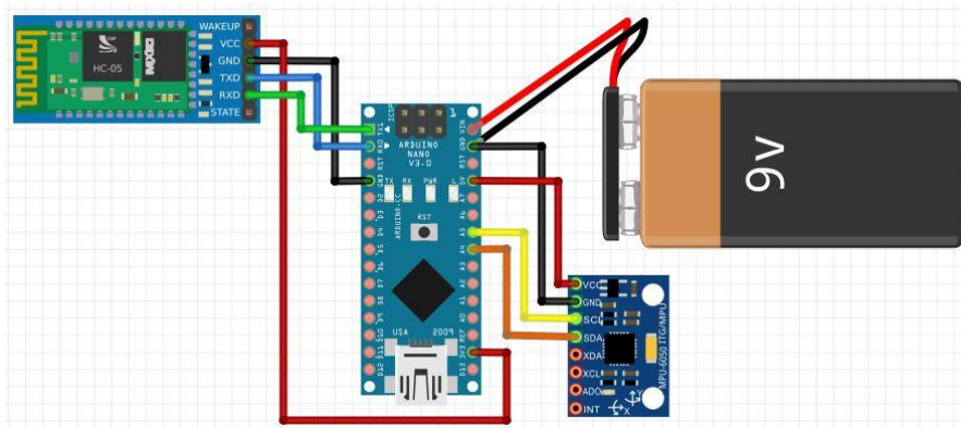
Figure 3. Design Hardware
