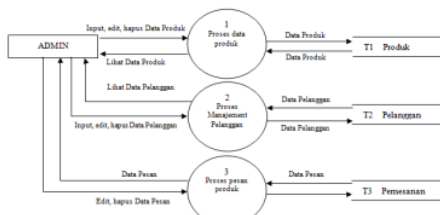
Gambar 4. Data Flow Diagram Admin
