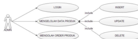
Gambar 2. Use Case Admin
