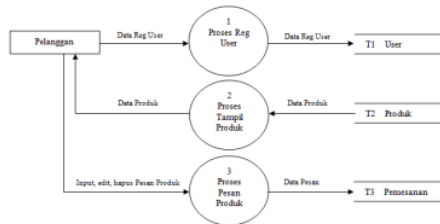
Gambar 5. Data Flow Diagram Pelanggan
