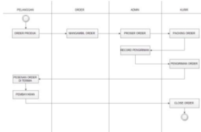
Gambar 3. Activity Diagram Proses Order
