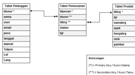
Gambar 6. Entity Relationship Diagram (ERD)
