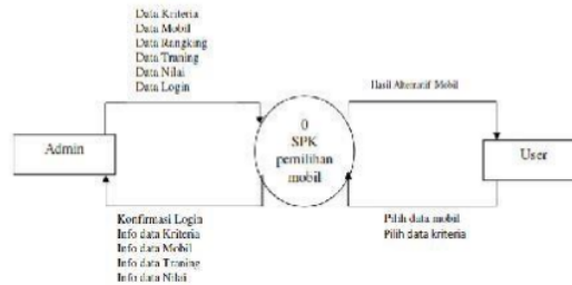
Gambar 1. DFD Level 0
